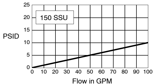
IN HF60074 Filter Performance
